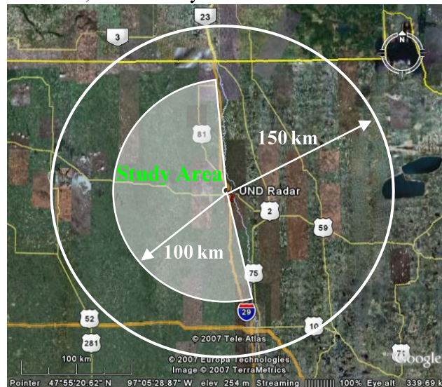
Figure 1: Study area for POLCAST4. The storms will be monitored by radar within the 150 km radius of the UND Radar. Hygroscopic seeding will be conducted within 100 km of the UND Radar, and west of the Red River of the North.
