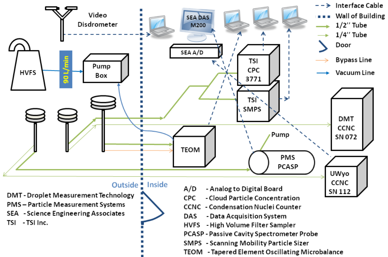
Figure 5. Diagram of how instruments will be setup for conducting surface measurement on the top of Clifford Hall.
