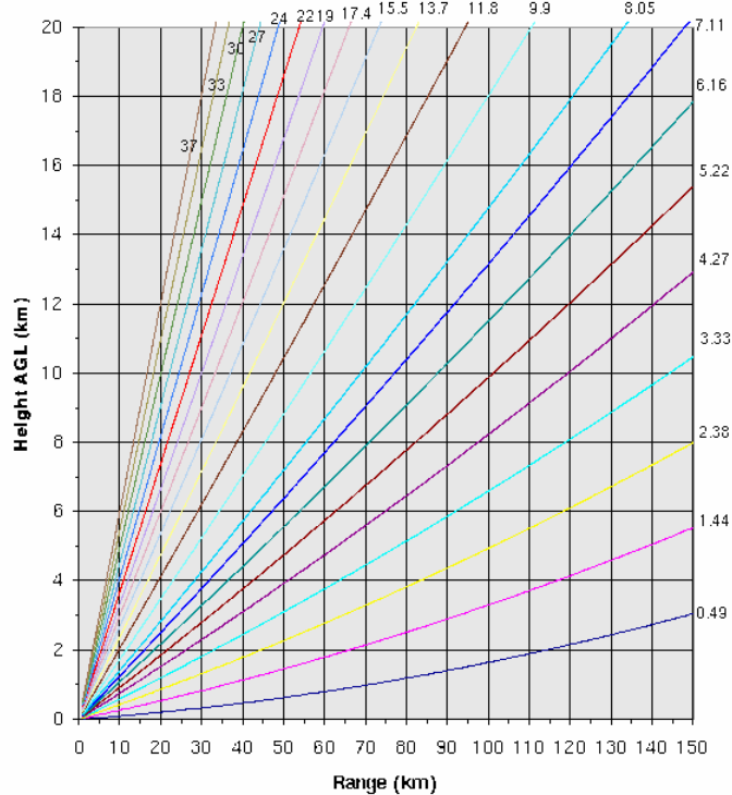
Figure 4: Range height diagram showing the location of possible elevation angles used in POLCAST4. We plan to use a reduced number of elevation angles (maximum 22^\circ for volume scan and 5.2^\circ for sector scans) to increase temporal resolution.
