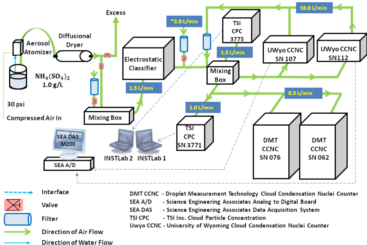
Figure 2: Laboratory configuration used to conduct performance checks on the Cloud Condensation Nuclei Counters.
